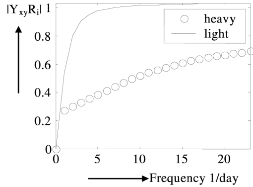
FIGURE 2.9. Cyclic admittance for different walls, L[49]
