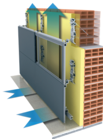
FIGURE 1.2. Wall cladding with ventilation corridor, L[14]
