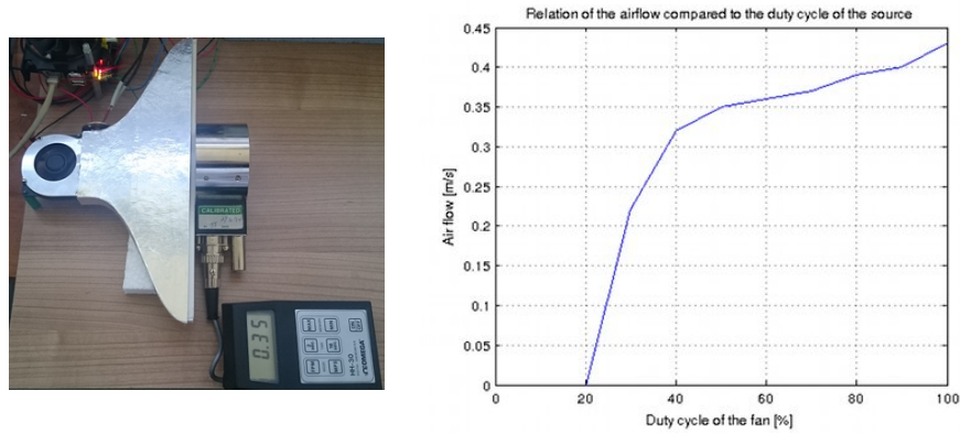
FIGURE 2.28. Air speed measurements a) Sensor position for measurement b) Obtained static characteristic
