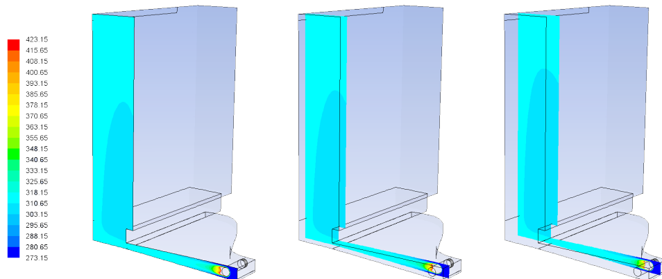
FIGURE 2.15. Temperatures [K] at y = \{0, 10, 20\} mm
