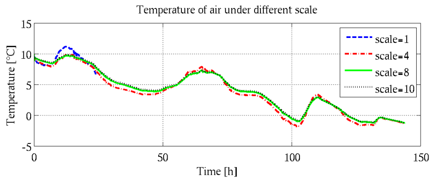
FIGURE 2.18. Influence of dimension variance in scale to air temperature in the zone
