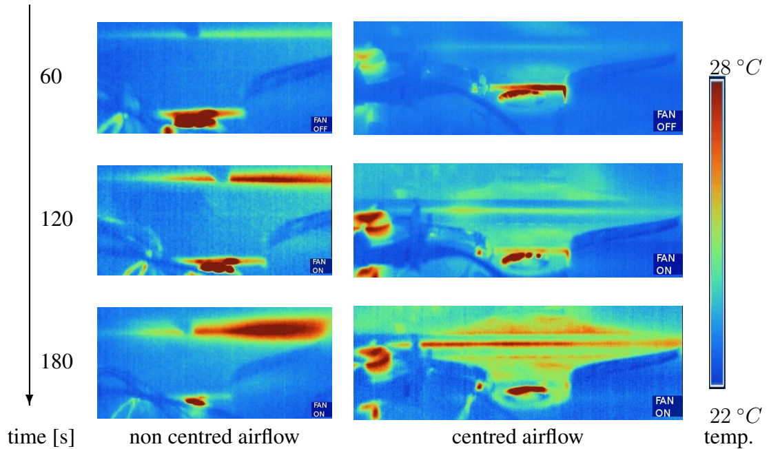
FIGURE 2.27. Thermo-visual tests
