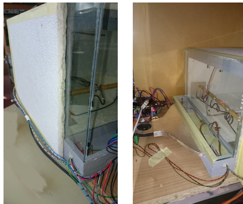
FIGURE 2.39. Parameter variation of scaled mock-up a) double thickness b) quadruple thickness
