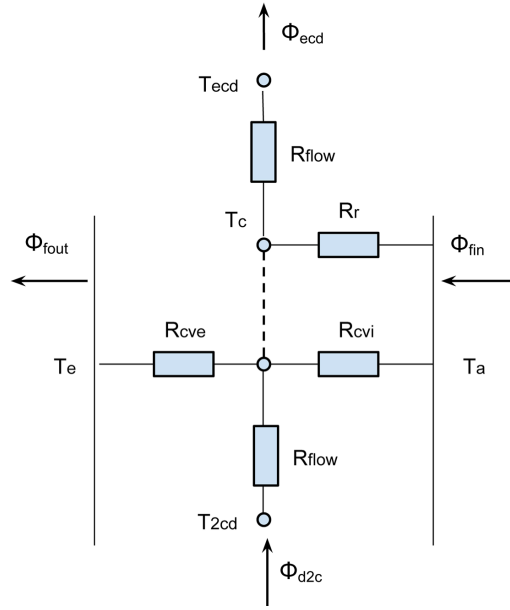
FIGURE 2.11. Thermal network of the corridor
